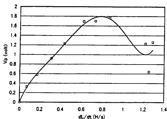
Fig. 7(c) Double coil (attraction mode)
